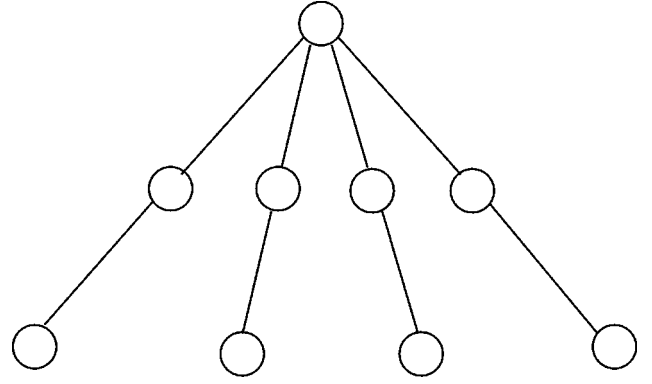
FIG. 2. The trivial ‘‘star’’ phylogeny. The path connecting two nodes always contains the tree root.
