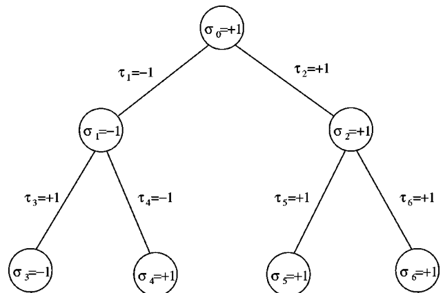
FIG. 1. The mutation process on a two-generation binary tree. The multiplicative variable \tau indicates whether a mutation occurred.
